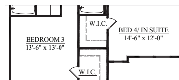
SECOND FLOOR PLAN ELEVATION B
