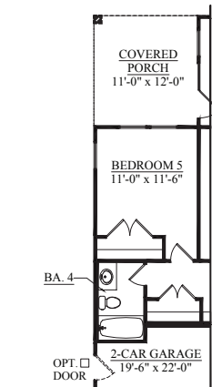
OPT. BED 5 W/ FULL BATH
