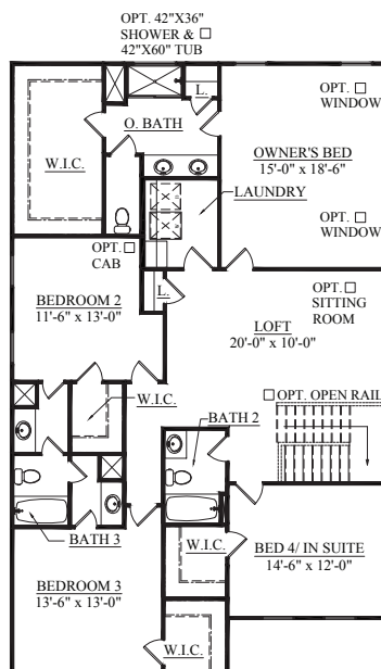
SECOND FLOOR PLAN ELEVATION A
