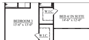
SECOND FLOOR PLAN ELEVATION C
