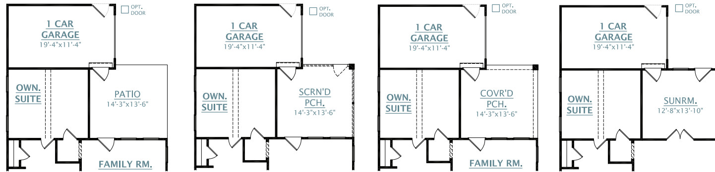
OPT. 1 CAR SIDELOAD GARAGE WITH PATIO OPT. 1 CAR SIDELOAD GARAGE WITH SCREEN PORCH OPT. 1 CAR SIDELOAD GARAGE WITH COVERED PORCH OPT. 1 CAR SIDELOAD GARAGE WITH SUNROOM
