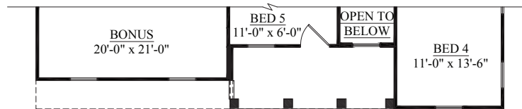
SECOND FLOOR PLAN ELEVATION D
