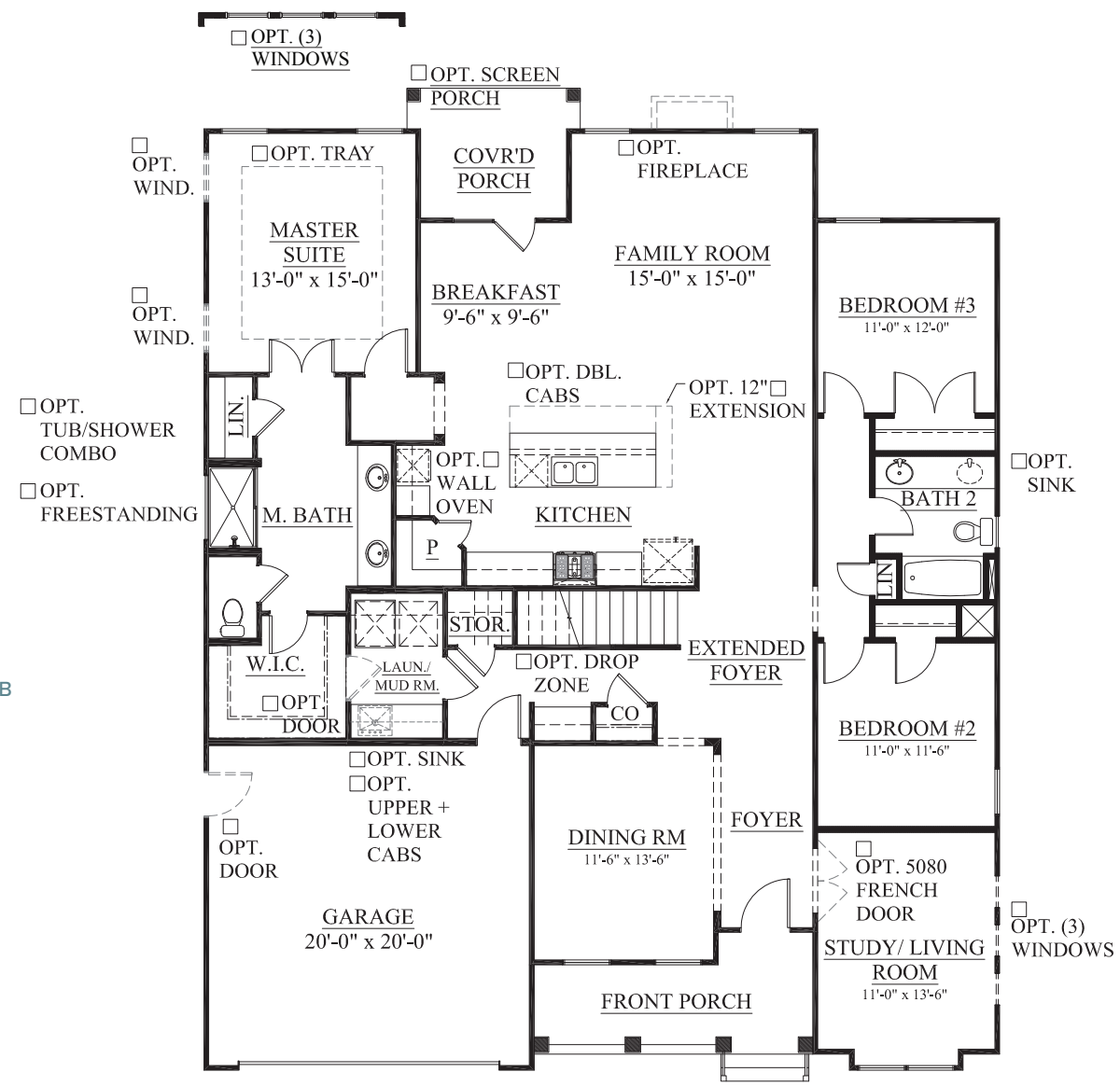
FIRST FLOOR PLAN ELEVATION A
