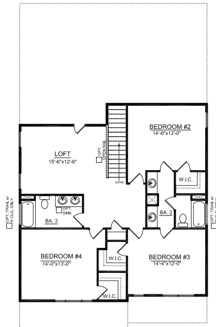
SECOND FLOOR PLAN ELEVATION A
