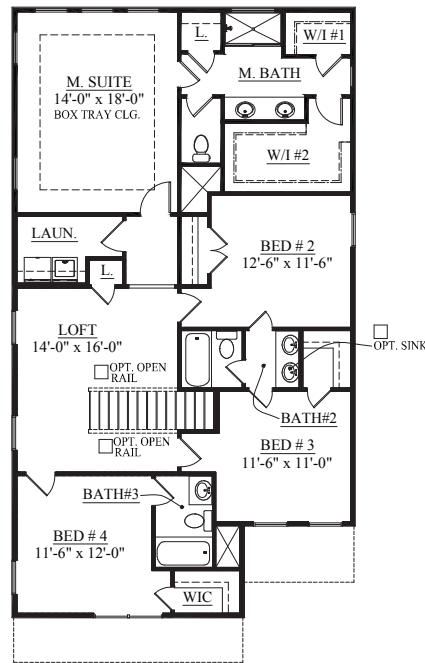
SECOND FLOOR PLAN ELEVATION A
