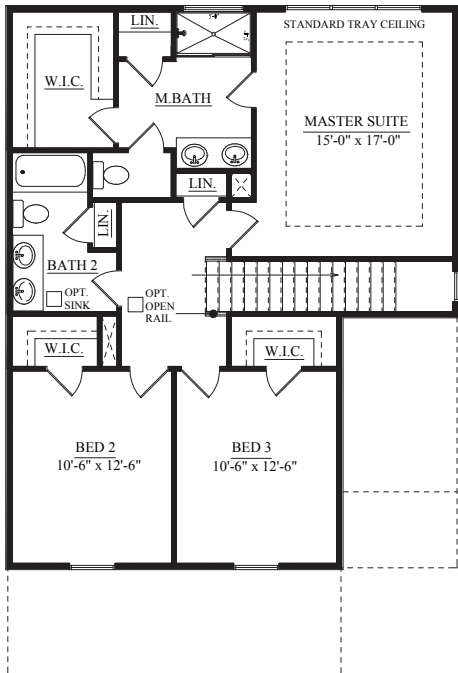
SECOND FLOOR PLAN ELEVATION A
