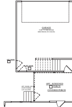
STD. GARAGE PLAN
