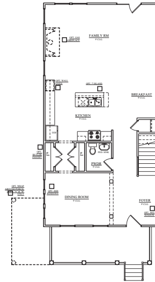
FIRST FLOOR PLAN ELEVATION A
