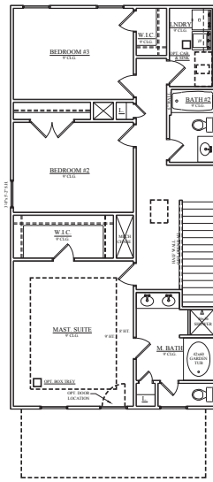
SECOND FLOOR PLAN ELEVATION A
