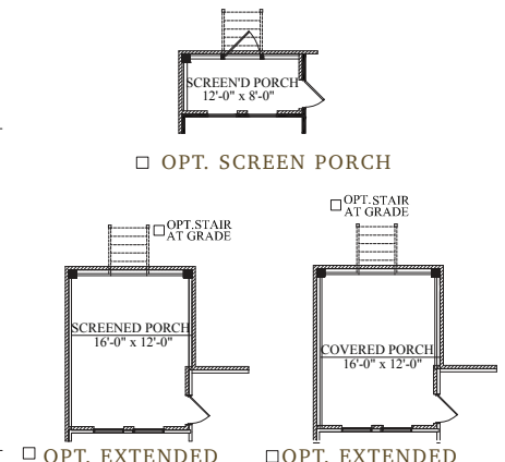
OPT. EXTENDED SCREEN PORCH OPT. EXTENDED COVERED PORCH
