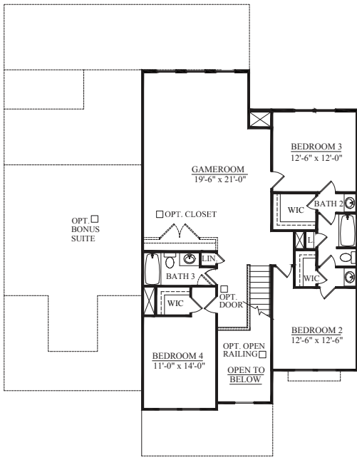
SECOND FLOOR PLAN ELEVATION A, C
