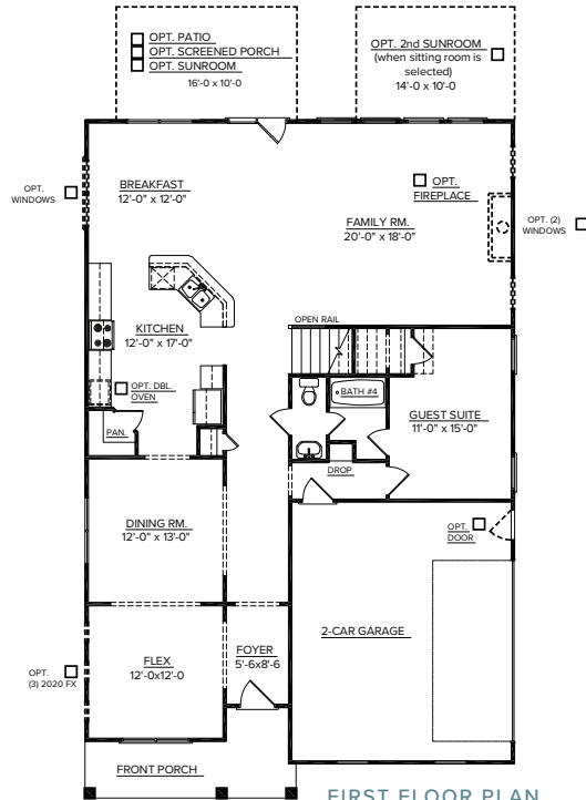
FIRST FLOOR PLAN ELEVATION A AND B
