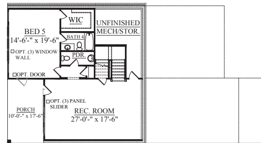
OPT. BASEMENT PLAN W/ REC ROOM AND BED 5
