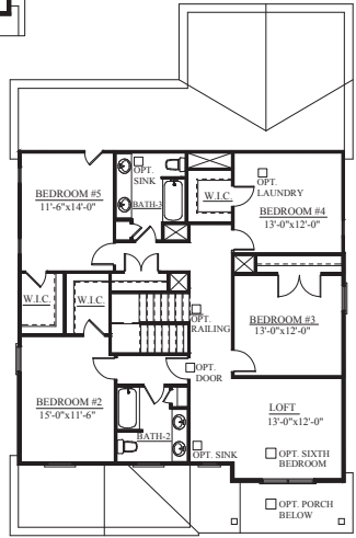
SECOND FLOOR PLAN ELEVATION A
