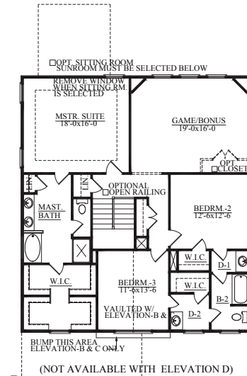
OPT. SECOND FLOOR PLAN WITH ENLARGED MASTER BATH AND JACK & JILL BATH
