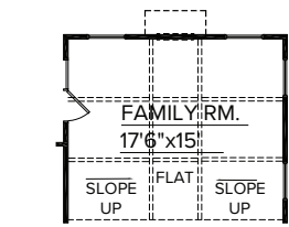
OPT. FAUX BEAM LAYOUT
