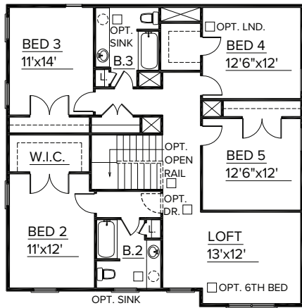
SECOND FLOOR PLAN ELEVATION A
