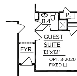
OPT GUEST SUITE SHOWN WITH ELEVATION A
