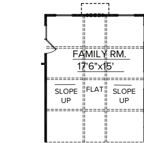
OPT. FAUX BEAM LAYOUT
