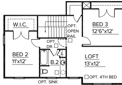
SECOND FLOOR PLAN ELEVATION A
