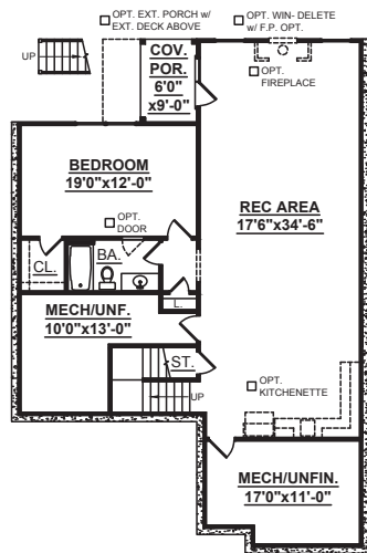
OPTIONAL FINISHED BASEMENT +1225 HEATED SQ FT
