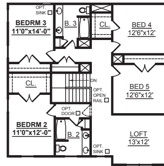
SECOND FLOOR PLAN ELEVATION A
