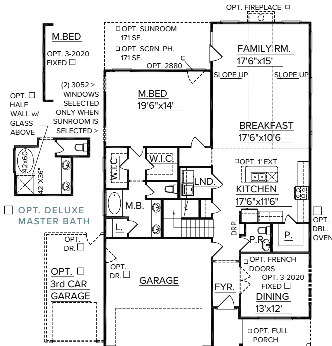
FIRST FLOOR PLAN ELEVATION A
