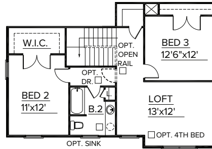
SECOND FLOOR PLAN ELEVATION A
