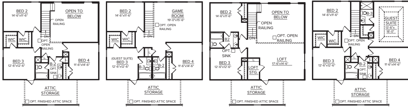
OPTIONAL OPEN SECOND FLOOR PLAN
