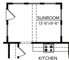
SUNROOM OPTION
