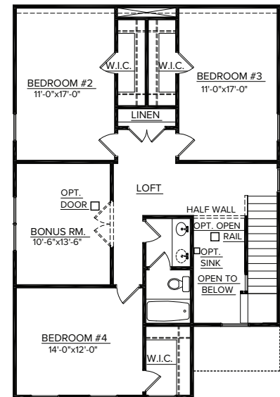
SECOND FLOOR PLAN ELEVATION A,B
