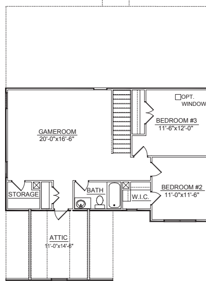
SECOND FLOOR PLAN ELEVATION A
