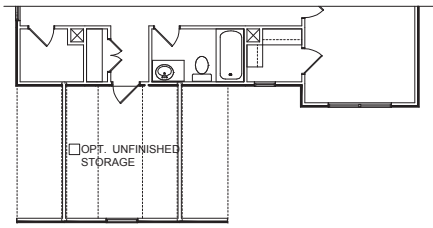
OPT. SECOND FLOOR PLAN W/ UNFINISHED STORAGE ELEVATION A
