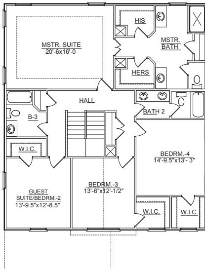
OPT. SECOND FLOOR PLAN WITH GUEST SUITE AND FULL BATH
