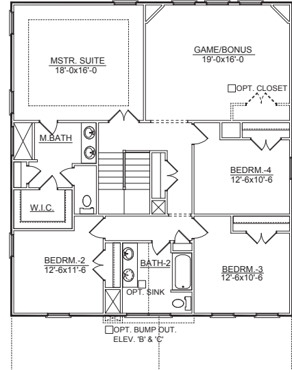
STANDARD SECOND FLOOR PLAN
