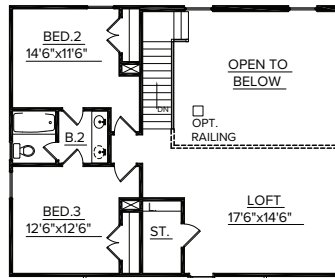
OPTIONAL OPEN SECOND FLOOR PLAN WITH LOFT
