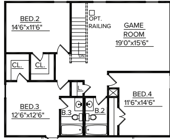
OPT SECOND FLOOR PLAN GUEST SUITE OPTION WITH GAMEROOM
