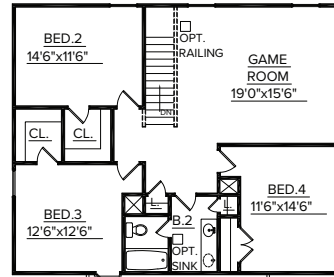
STANDARD FULL SECOND FLOOR PLAN WITH GAME RM.
