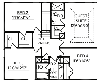
OPTIONAL FULL SECOND FLOOR PLAN WITH GUEST SUITE
