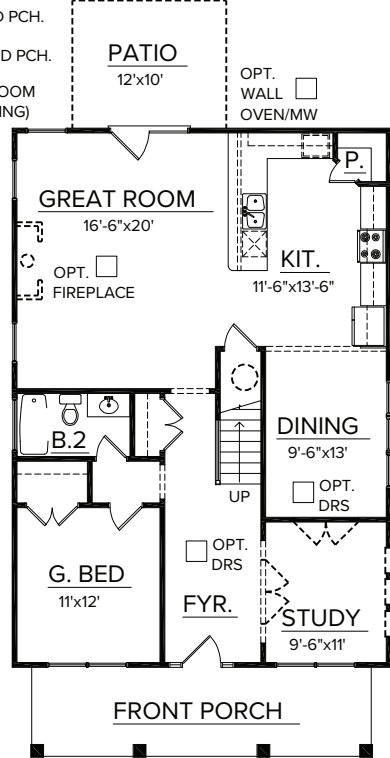
FIRST FLOOR PLAN ELEVATION A
