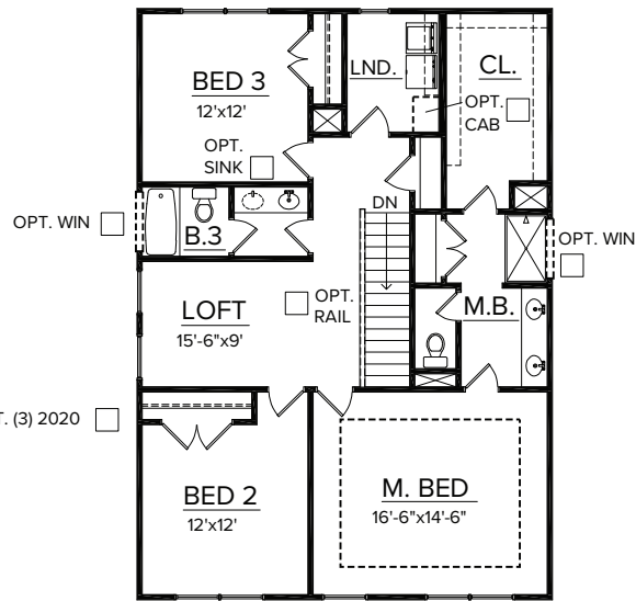
SECOND FLOOR OPT. 3 BEDROOM WITH LOFT PLAN
