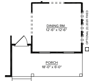
□ MAIN LEVEL PLAN ELEVATION C
