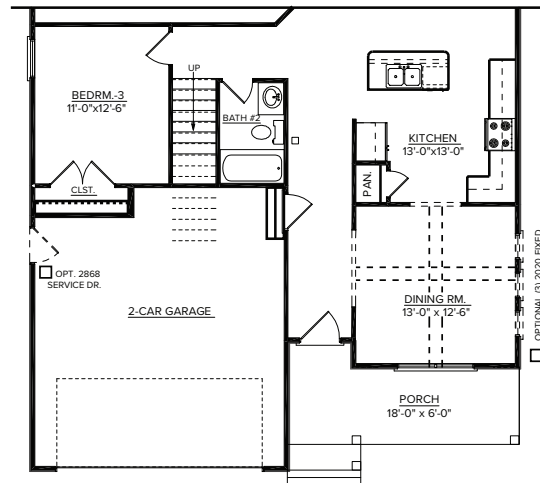
MAIN LEVEL PLAN WITH BONUS ROOM
