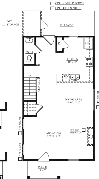
MAIN LEVEL PLAN ELEVATION D
