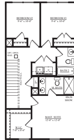
UPPER LEVEL PLAN THREE BEDROOM OPT.- ADD 50 SF ELEVATION D, E, F
