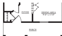
MAIN LEVEL PLAN 3-BEDRM OPT. ONLY ELEVATION A, B
