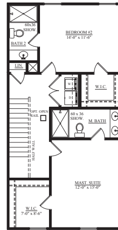
UPPER LEVEL PLAN TWO BEDROOM- ADD 50 SF ELEVATION D, E, F
