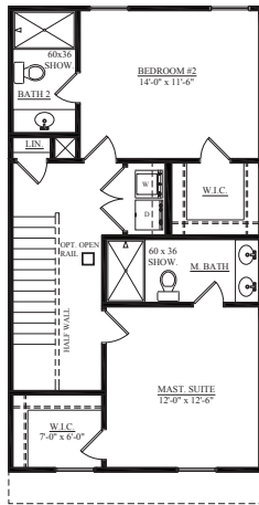
UPPER LEVEL PLAN ELEVATION A, B
