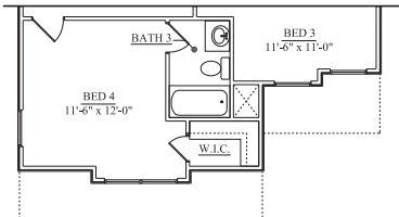
SECOND FLOOR PLAN ELEVATION C
