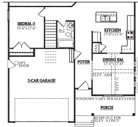
MAIN LEVEL PLAN WITH BONUS ROOM
