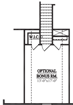
OPT. BONUS ROOM ELEVATION A, C
