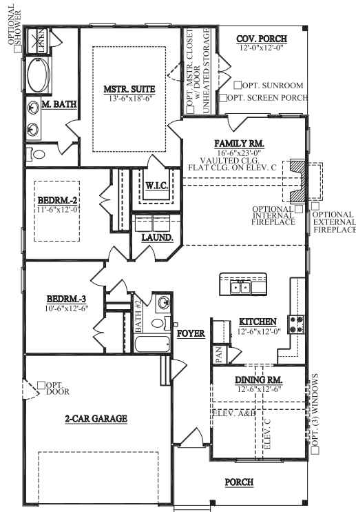
MAIN LEVEL PLAN ELEVATION A, B
