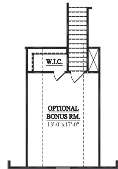
OPT. BONUS ROOM ELEVATION B
