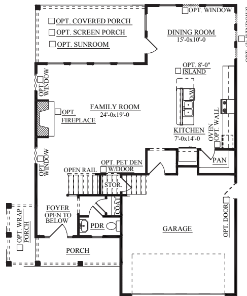
FIRST FLOOR PLAN ELEVATION A
