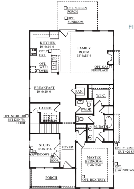
FIRST FLOOR PLAN ELEVATION A
