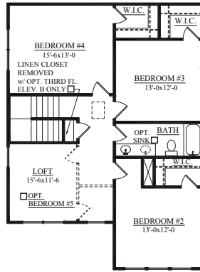
SECOND FLOOR PLAN ELEVATION A
