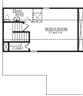
OPT. 3RD FLOOR PLAN ELEVATION B, D, G ONLY
