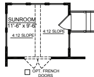
SUNROOM OPTION #1
