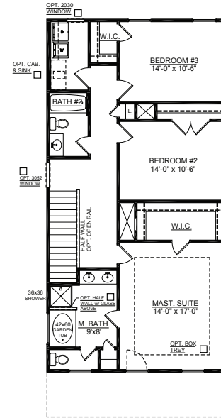
UPPER LEVEL PLAN ELEVATION A
