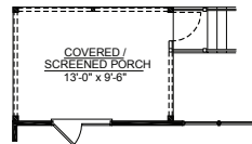
COVERED/ SCREEN PORCH OPTION
