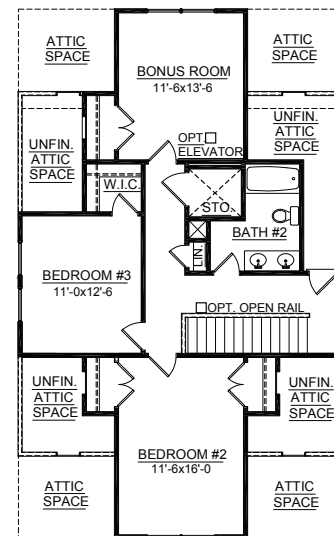
STANDARD UPPER LEVEL PLAN ELEVATION A
