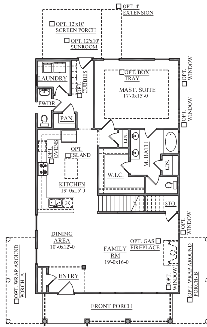
FIRST FLOOR PLAN ELEVATION A,B,C
