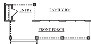
FRONT PORCH ELEVATION B,C,D
