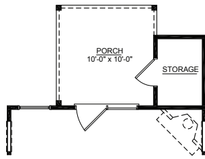
COVERED/ SCREEN PORCH W/ STORAGE ROOM OPTION
