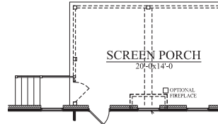
OPT. SCREEN PORCH
