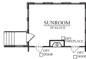
OPT. SUNROOM
