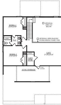
OPTIONAL OPEN SECOND FLOOR PLAN
