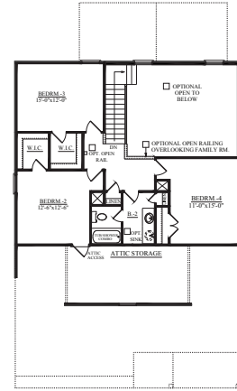
OPTIONAL SECOND FLOOR PLAN WITH BEDROOM-4
