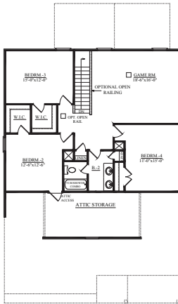
STANDARD FULL SECOND FLOOR PLAN WITH GAME RM.
