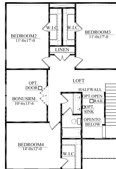
SECOND FLOOR PLAN ELEVATION A, B
