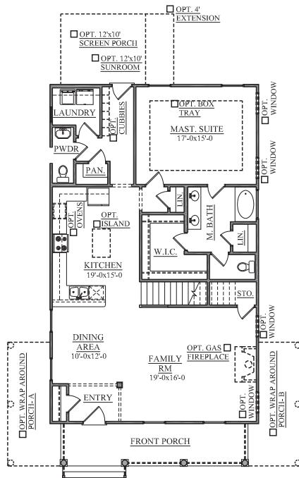
FIRST FLOOR PLAN ELEVATION A,B,C
