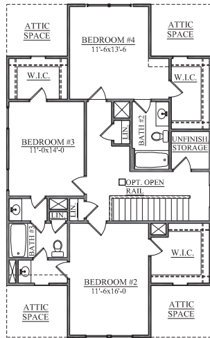
4TH BEDROOM UPPER LEVEL PLAN - OPT 2
