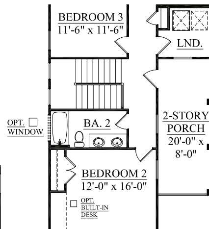
Second Floor Plan ELEVATION B, C
