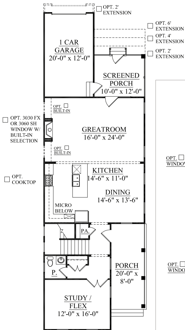
First Floor Plan ELEVATION A, B, C
