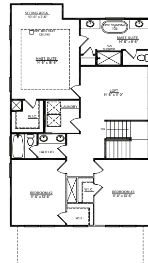
SECOND FLOOR PLAN ELEVATION A
