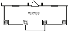
FIRST FLOOR PORCH ELEVATION B
