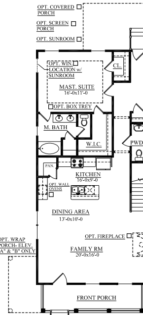
MAIN LEVEL PLAN-ELEVATION "A"
