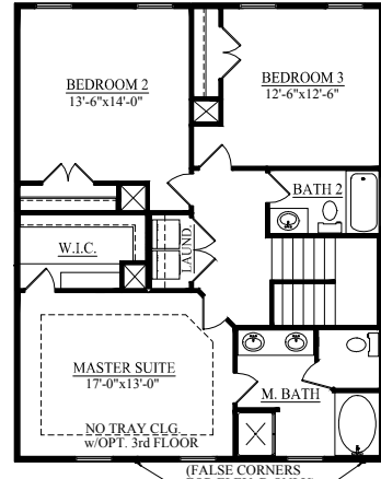
□ OPTIONAL DELUXE MASTER SECOND FLOOR PLAN "A&D"
