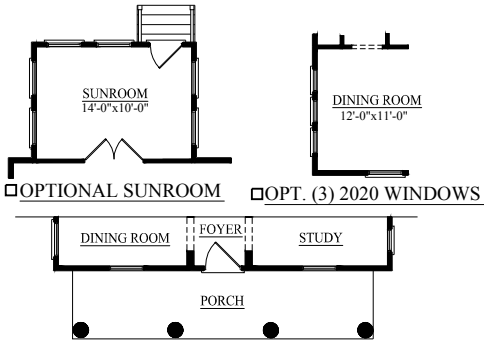
□ OPTIONAL SUNROOM □ OPT. (3) 2020 WINDOWS
