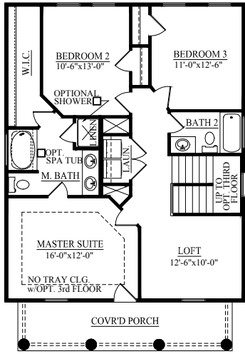
□ STANDARD SECOND FLOOR PLAN "B&C"
