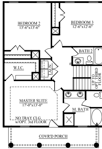
□ OPTIONAL DELUXE MASTER SECOND FLOOR PLAN "B&C"
