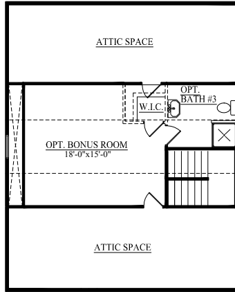
□ OPT. THIRD FLOOR PLAN "B" & "C"
