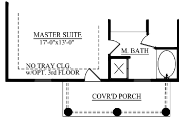
□ OPTIONAL DELUXE MASTER SECOND FLOOR PLAN "E"
