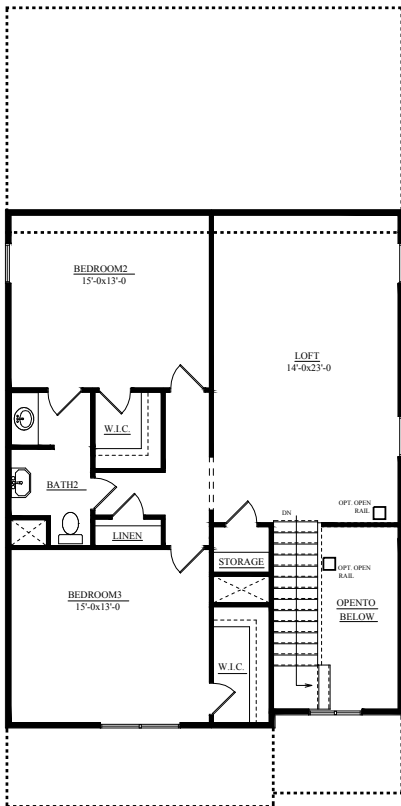
SECOND FLOOR LEVEL A
