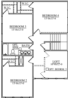
SECOND FLOOR PLAN ELEV. A
