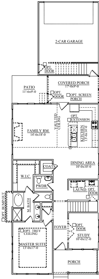
FIRST FLOOR PLAN ELEV. A
