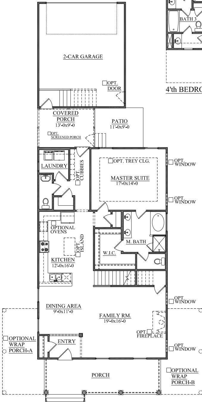
FIRST FLOOR PLAN ELEV. A,B&C
