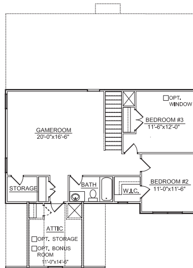
SECOND FLOOR PLAN ELEVATION A
