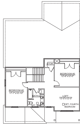
SECOND FLOOR PLAN ELEVATION A
