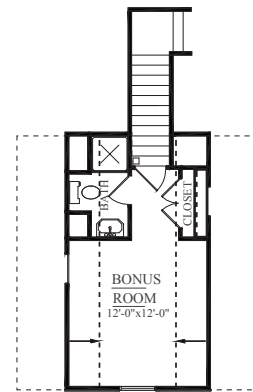
OPTIONAL BONUS ROOM WITH BATH STANDARD WITH ELEVATION D ADD 247 SF HEATED
