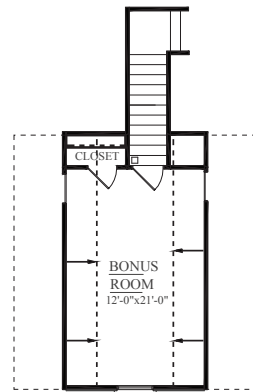
OPTIONAL BONUS ROOM ADD 247 SF HEATED
