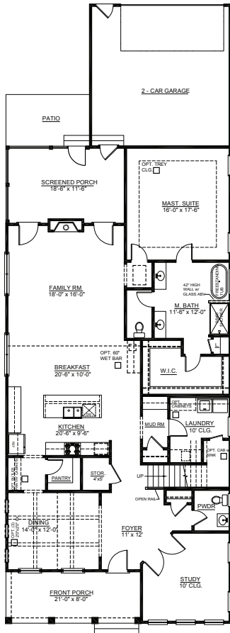
FIRST LEVEL PLAN
