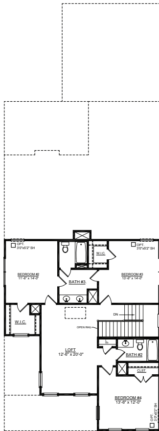
UPPER LEVEL PLAN
