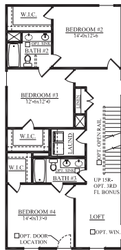
OPT. 4TH BEDROOM WITH LOFT
