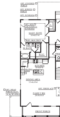
FIRST FLOOR PLAN ELEVATION A
