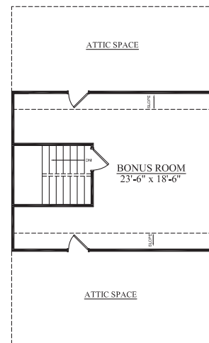
OPTIONAL 3RD FLOOR PLAN
