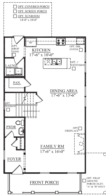
MAIN LEVEL PLAN ELEVATION A
